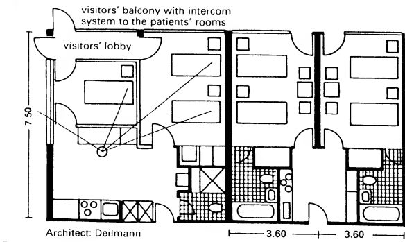
2 Care of infectious children: room variations Architect: Deilmann
